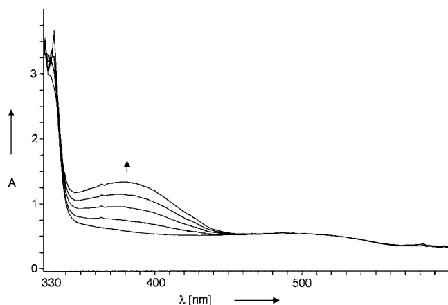
Figure 1. UV/Vis spectra showing the formation of carbonyl oxide 1b in an organic glass; irradiation ( \lambda > 515 nm) of diazomethane 5b dissolved in oxygen-saturated \text{CCl}_3\text{F}/(\text{CBrF}_2)_2 (1:1) at 78 K; the absorption with a maximum at 380 nm is growing in
