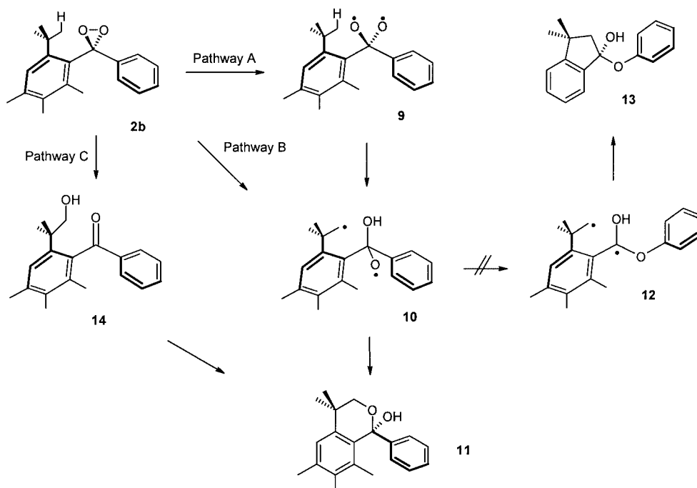
Scheme 3. Mechanisms for the thermal decay of dioxirane 2b
