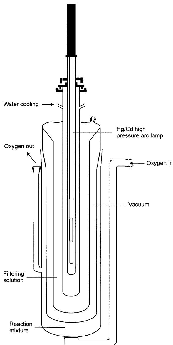
Figure 4. Photoreactor for the synthesis of dioxirane 2b
