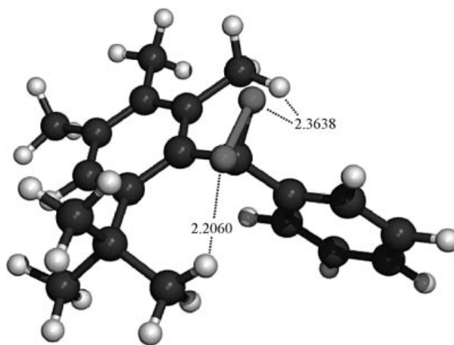
Figure 6. Structure of dioxirane 2b calculated at the B3LYP/6-31G(d,p) level of theory
