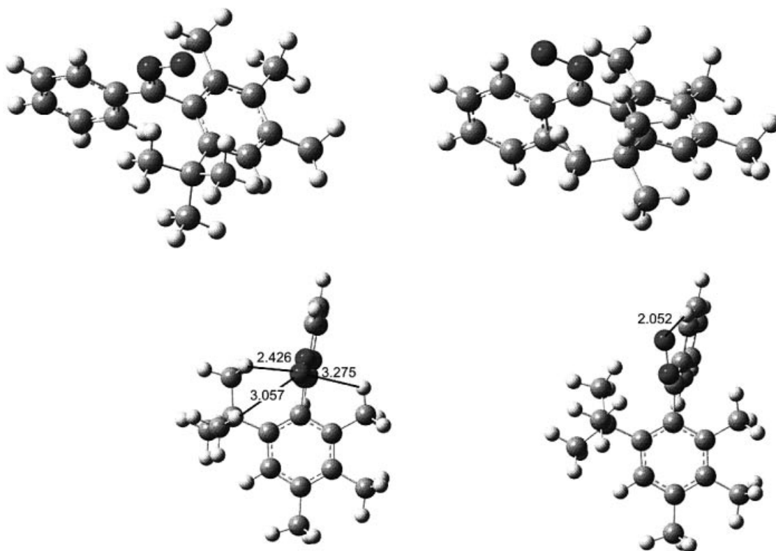
Figure 3. Structure of carbonyl oxides 1b calculated at the B3LYP/6-31G(d) level of theory; right hand side: conformer syn-A ; left hand side: conformer syn-B
