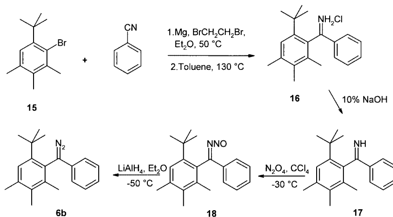
Scheme 1. Synthesis of diazo compound 6b
