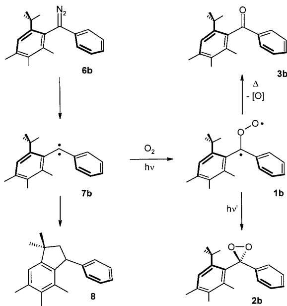
Scheme 2. Synthesis of carbonyl oxide 1b and dioxirane 2b by photooxidation of diazo compound 6b
