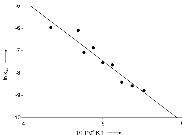
Figure 2. Arrhenius plot of the thermal decay of carbonyl oxide 1b in \text{CCl}_3\text{F}/(\text{CBrF}_2)_2 (1:1) in the temperature range between 181 and 230 K; the decrease of the strong absorption with \lambda_{\text{max}} = 380 nm is monitored
